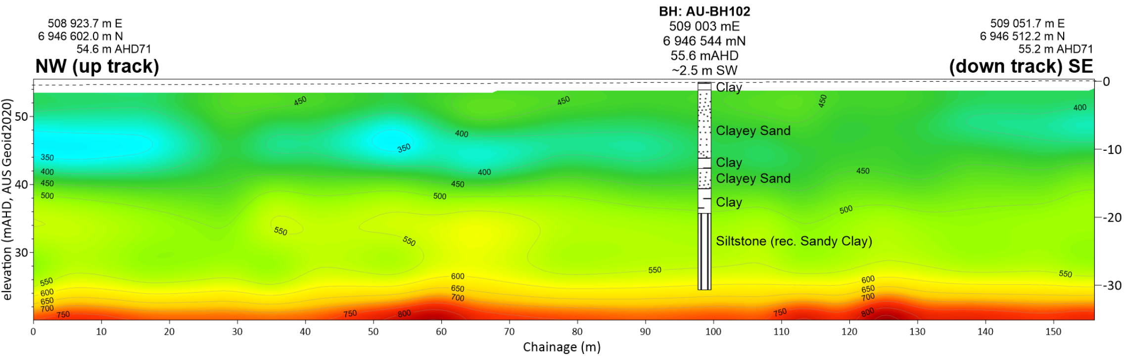
Seismic Line MASW AU-GP 101
